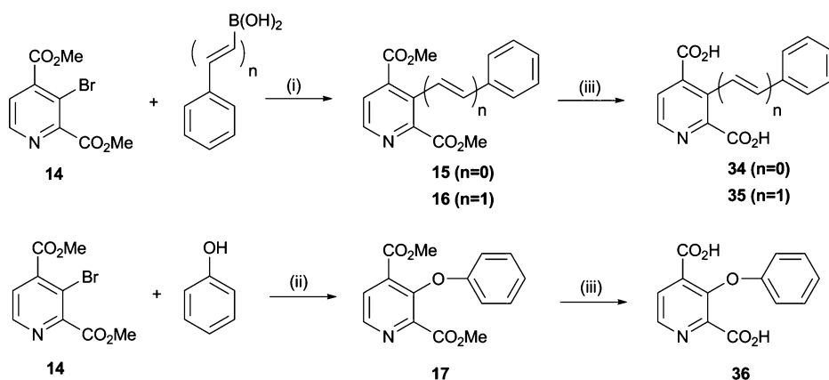
Scheme 3 Synthesis of pyridine dicarboxylate derivatives 34–36 . Reagents and conditions: (i) Pd(OAc) 2 (10 mol%), PPh 3 (0.2 eq.), Cs 2 CO 3 (1.1 eq.), DMF, 70 °C, 3–5 h, 60–75%; (ii) CuI (0.1 eq.), N -( n -butyl)imidazole (0.5 eq.), Cs 2 CO 3 (2 eq.), toluene, MW, 140 °C, 1 h, 44%; (iii) NaOH, MeOH, H 2 O, 6 h–overnight, 49–75%.
