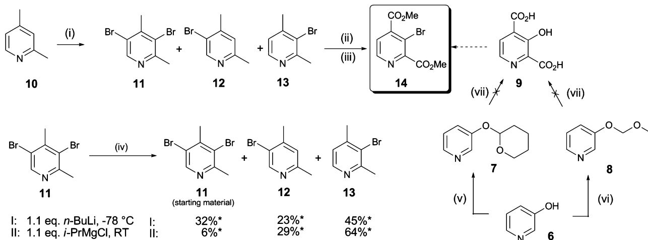
Scheme 2 Synthesis of 3-bromopyridine 14 . Reagents and conditions: (i) Br 2 (0.9 eq.), 20% oleum, 165 °C, 24 h, 11 (12%), 12 (22%), 13 (35%); (ii) KMnO 4 (5 eq.), NaOH (0.7 eq.), H 2 O, 110 °C, 3 h; (iii) cat. H 2 SO 4 , MeOH, reflux, 24 h, 53%; (iv) n -BuLi (1.1 eq.), THF, -78 °C, 1 h, or i -PrMgCl (1.1 eq.), THF, RT; then MeOH workup; (v) tetrahydropyran-2-ol (1.1 eq.), PPh 3 (1.1 eq.), diisopropyl azodicarboxylate (1.1 eq.), RT, 2 h, 46%; 23 (vi) methoxymethyl chloride (1.05 eq.), KO t Bu (1.1 eq.), DMF-CH 3 CN, RT, 1 h; 26 (vii) base (1.5 eq.), then excess CO 2 (s); base (1.5 eq.), then excess CO 2 (s); then HCl/dioxane; *Ratios as determined by 1 H NMR.
