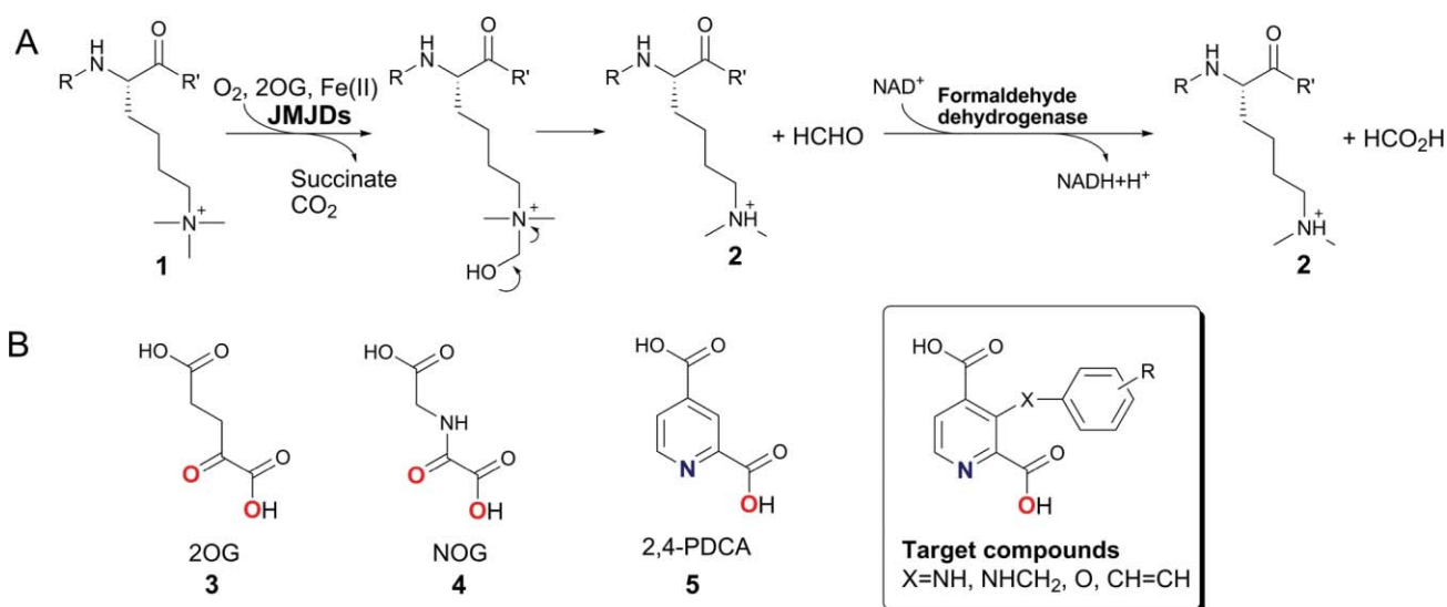
Scheme 1 A. The N^\epsilon -methyl lysine demethylation reaction catalysed by the 2OG-dependent JMJD2 histone demethylases, which preferentially act on tri- and di- N^\epsilon -methylated lysines. Demethylation of N^\epsilon -trimethyllysyl residues ( 1 ) proceeds via hydroxylation to give an unstable hemiaminal intermediate, which collapses spontaneously to release the demethylation product 2 . The formation of the by-product formaldehyde can be measured spectrophotometrically using formaldehyde dehydrogenase and \text{NAD}^+ in a coupled enzymatic assay. B. Structures of the 2OG cosubstrate ( 3 ), its analogues NOG ( 4 ) and 2,4-PDCA ( 5 ), and the targeted C-3 substituted 2,4-PDCA derivatives. The ligand atoms involved in chelation of the ferrous iron are shown in red and blue.
