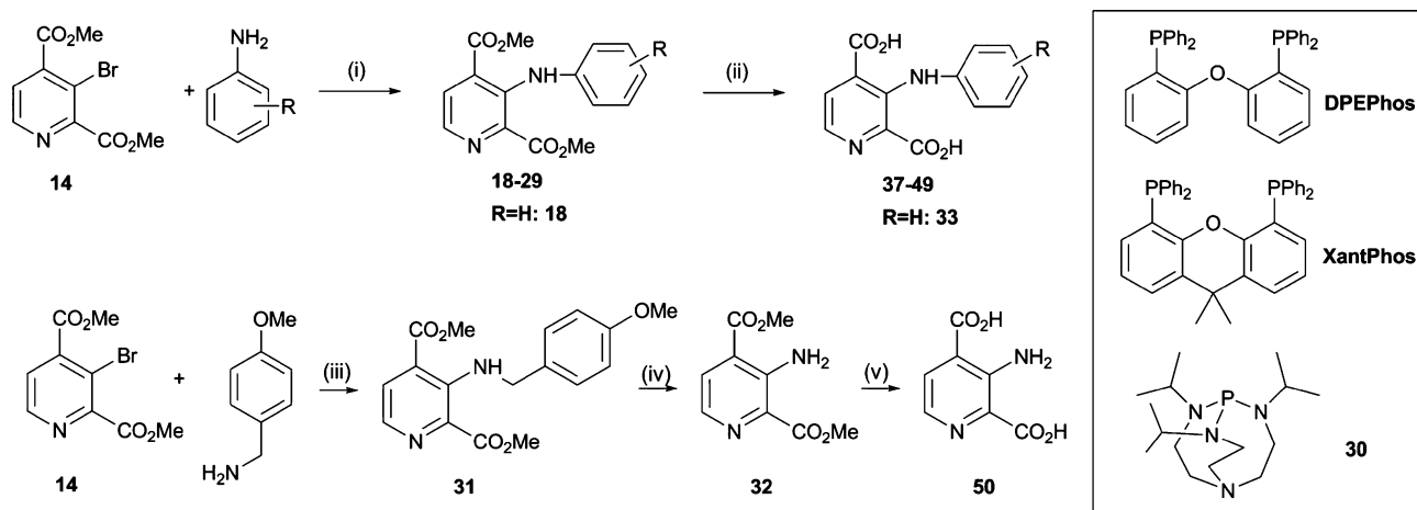
Scheme 4 Synthesis of pyridine dicarboxylate derivatives 37–50 . Reagents and conditions: (i) Pd 2 dba 3 (2 mol%), ligand L (6 mol%), base (1.4 eq.), toluene, MW, 110–150 °C; L = PPh 3 or BINAP or 30 : <5% conversion; L = DPEPhos: 11% yield; L = XantPhos: 77% yield; (ii) NaOH, MeOH–H 2 O, RT; (iii) Pd 2 dba 3 (2 mol%), XantPhos (6 mol%), Cs 2 CO 3 (1.4 eq.), toluene, MW, 110 °C, 12 h, 69%; (iv) CF 3 CO 2 H, CH 2 Cl 2 , 0 °C to RT, 89%; (v) NaOH, MeOH–H 2 O, 2 h, RT, 67%.
